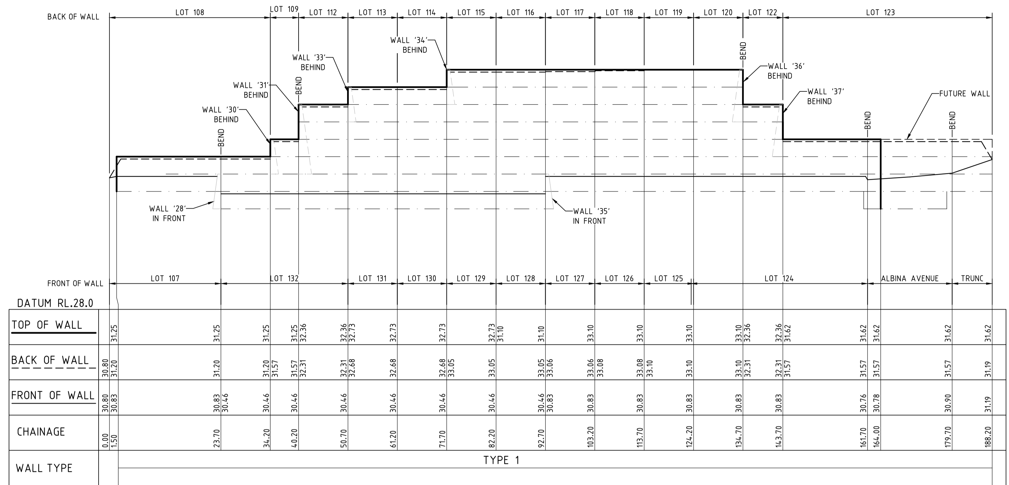
RETAINING WALL '32' HORIZ - 1:500 VERT - 1:50
