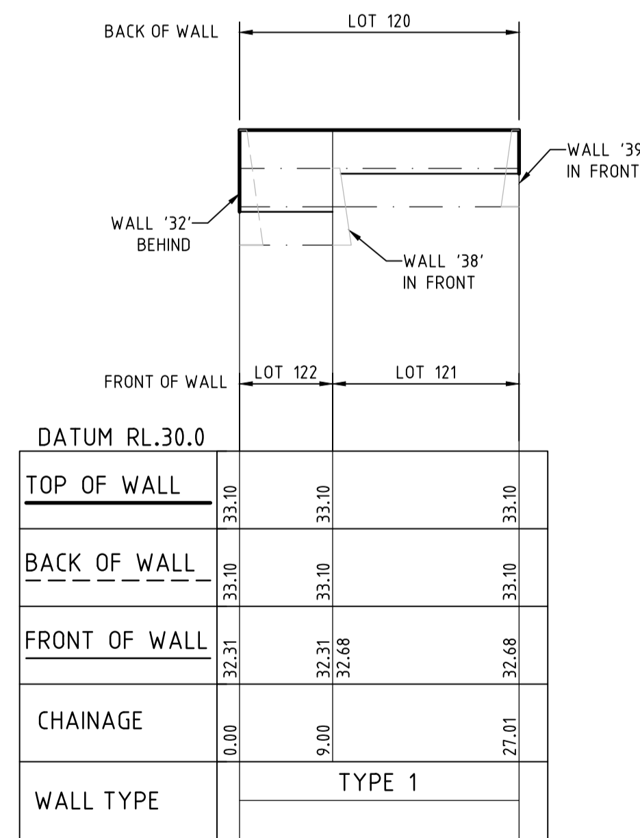
RETAINING WALL '36' HORIZ - 1:500 VERT - 1:50
