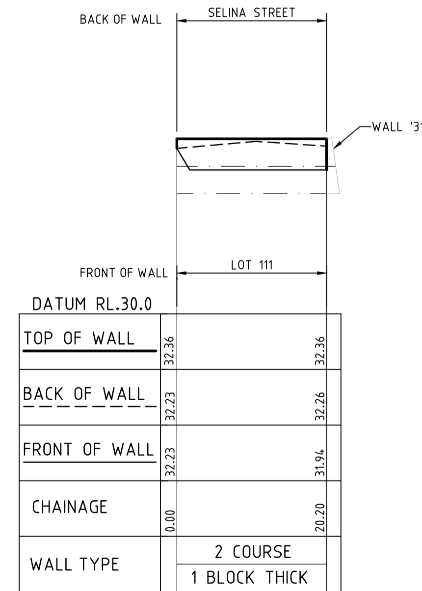
RETAINING WALL '46' HORIZ - 1:500 VERT - 1:50
